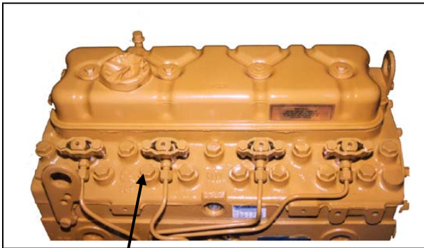
4.248 smaller injectors installed parallel to valve cover
